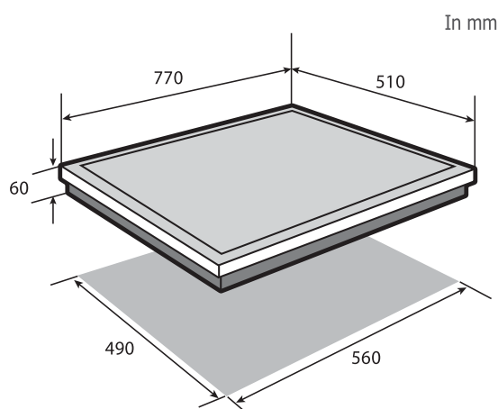
Installation Diagram BP1184HUB
